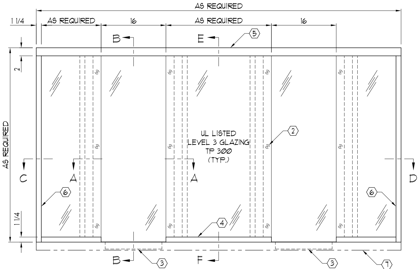
ELEVATION ( - REQUIRED)
