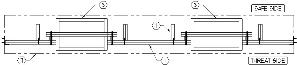
PLAN VIEW
