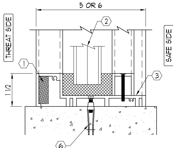
SECTION B
