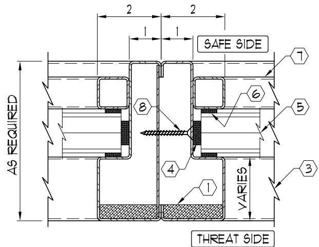
SECTION B
