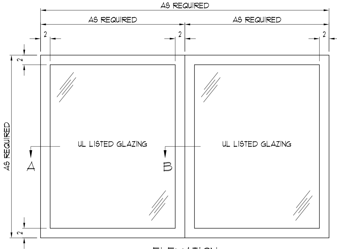
ELEVATION ( _ - REQUIRED )
