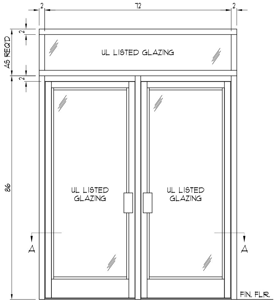
ELEVATION (__ - REQUIRED)
